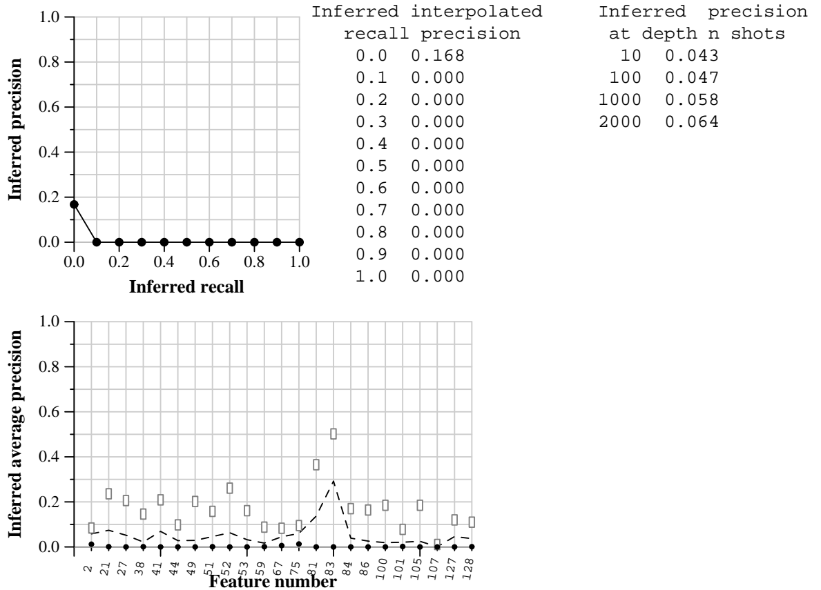
Run score (dot) versus median (---) versus best (box) by feature
