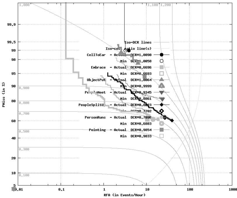
DET for SED12_CMU-IBM_interactiveED_EVAL12_2 : CMU-IBM_2012_interactiveED_EVAL12_ENG_s-camera_c-FVNoSkip_1
