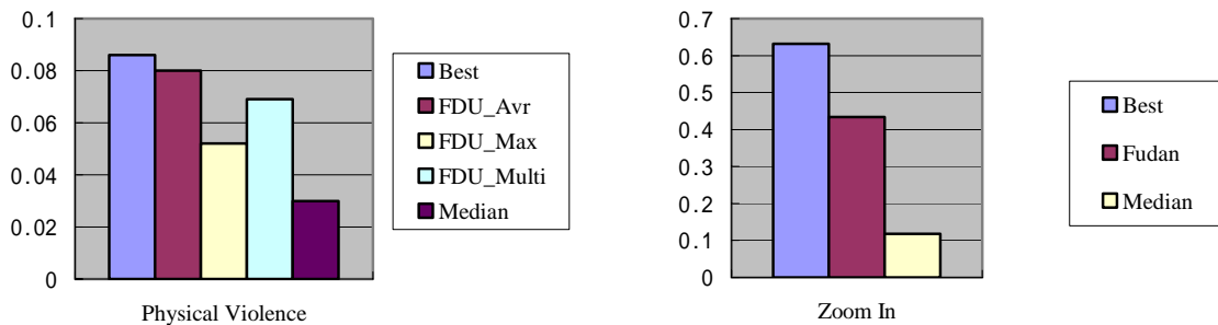
Figure 6. Motion feature extraction Evaluation (Average Precision)
