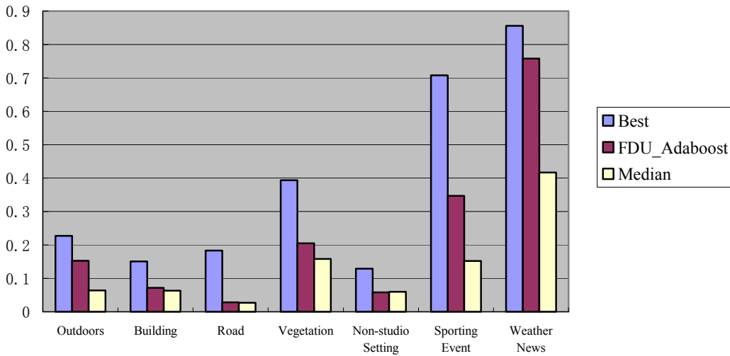
Figure 1. General Scene feature extraction Evaluation (Average Precision)
