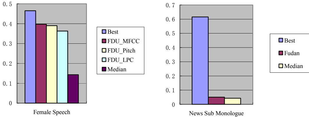
Figure 4. Audio feature extraction Evaluation (Average Precision)
