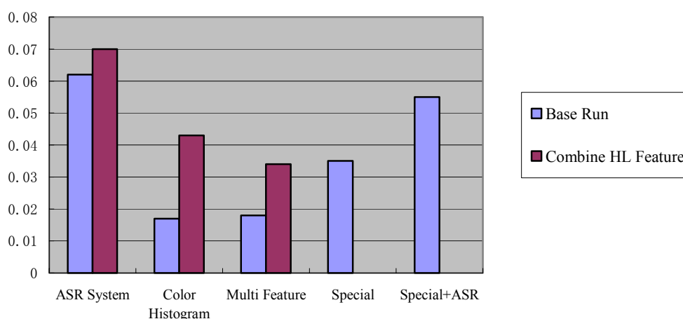
Figure 6. Comparison between Base run and High-level Feature Run (Mean Average Precision)
