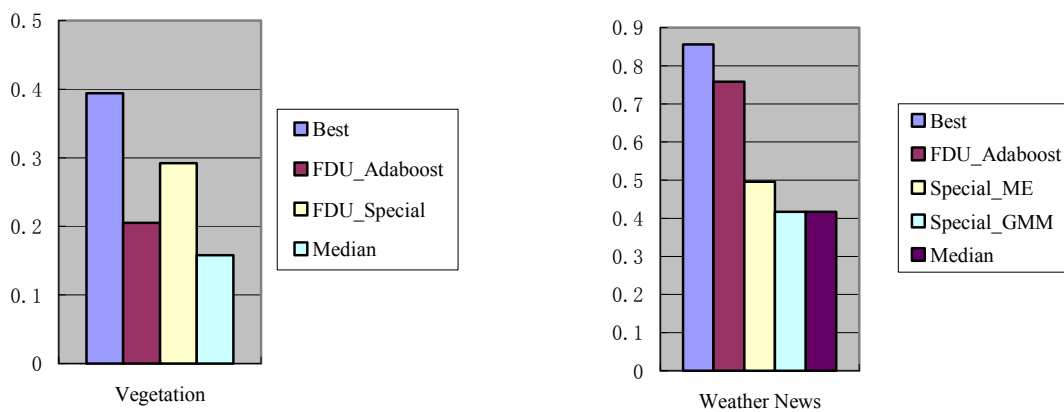
Figure 2. Special Scene feature extraction Evaluation (Average Precision)
