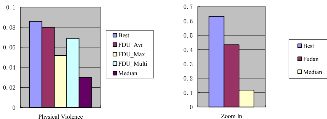
Figure 5. Motion feature extraction Evaluation (Average Precision)
