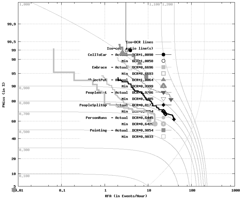
DET for SED12_CMU-IBM_interactiveED_EVAL12_2 : CMU-IBM_2012_interactiveED_EVAL12_ENG_s-camera_p-FVSkip_2
