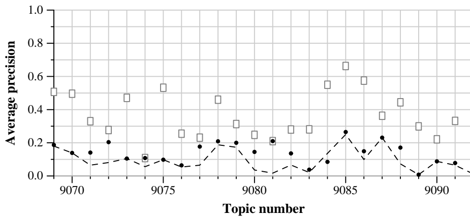
Run score (dot) versus median (---) versus best (box) by topic
